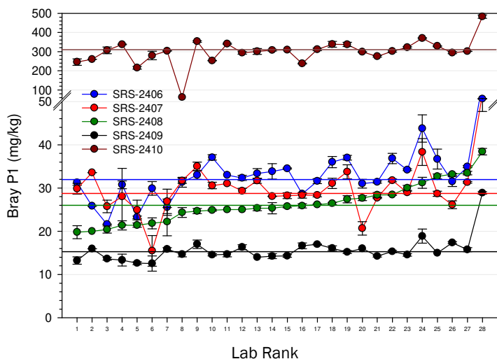
Figure 2. Bray P1 distribution plots for SRS materials, ALP 2024 Cycle 54.
